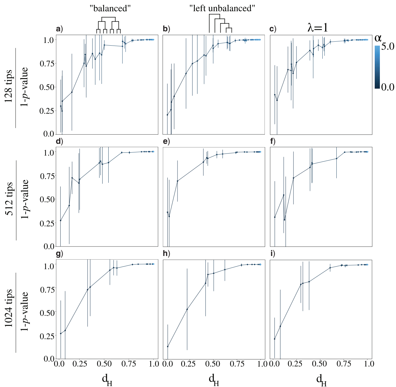
FIGURE 5. Investigating the relationship between model distances and the significance of likelihood ratio tests between fitted BM and OU models (traits simulated under an OU model). Results shown for three different tree shapes: “balanced” (left panels), “left unbalanced” (center), and trees simulated under a Yule model with the birth rate \lambda = 1 (right) with equal branch lengths that are scaled to give a total tree height of 1.0. P values for a likelihood ratio test comparing the OU and BM models as a function of their Hellinger distance ( d_H ) are shown for three different tree sizes: 128 (a–c), 512 (d–f), and 1024 (g–i) tips. The mean (circle) and standard deviations (bars) of the distribution of 10 replicate P values (subtracted from one). Each simulation replicate was computed by incrementally increasing the \alpha parameter of the OU model from 0 to 5 (from left to right in each panel colored in the blue scale shown), at increments of 0.01.
